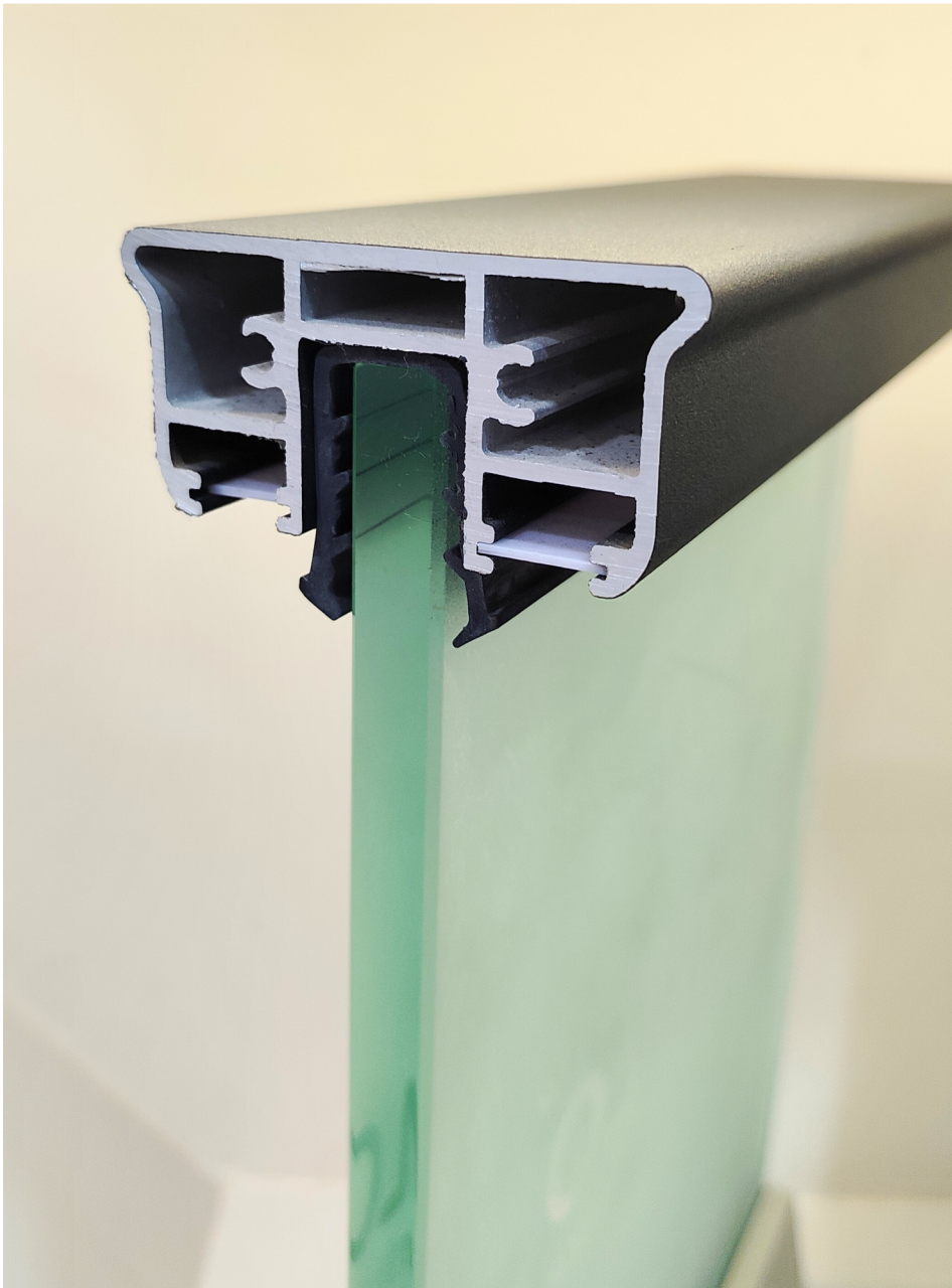
Curved Edge Led 31 × 68 mm
